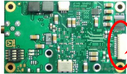
J5, CVBS output (available with MP110M-VC only)
